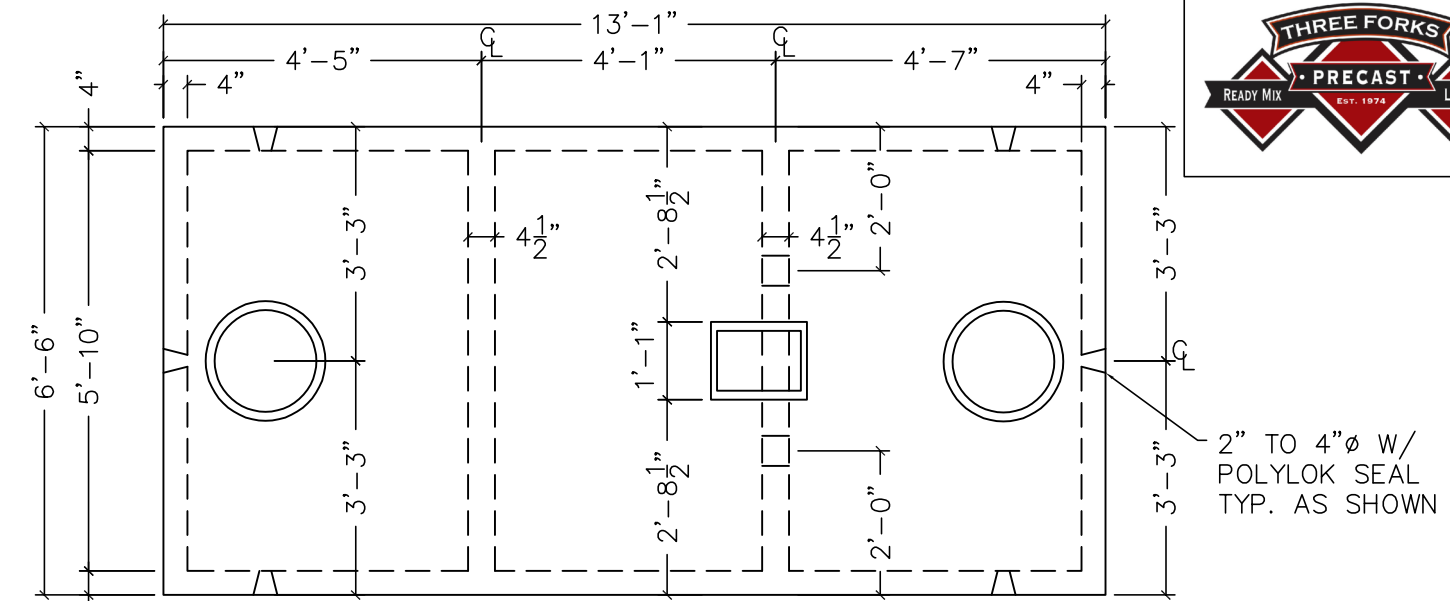
TOP VIEW
