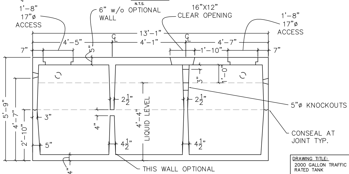
SECTION VIEW
